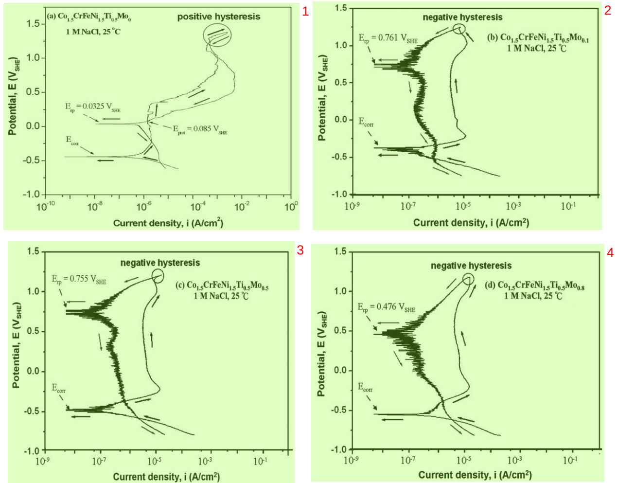
Fig. 5. Cyclic polarisation curves of the \text{Co}_{1.5}\text{CrFeNi}_{1.5}\text{Ti}_{0.5}\text{Mo}_x alloys with various Mo contents (a) x = 0 , (b) x = 0.1 , (c) x = 0.5 , and (d) x = 0.8 mol in deaerated 1 M NaCl.
