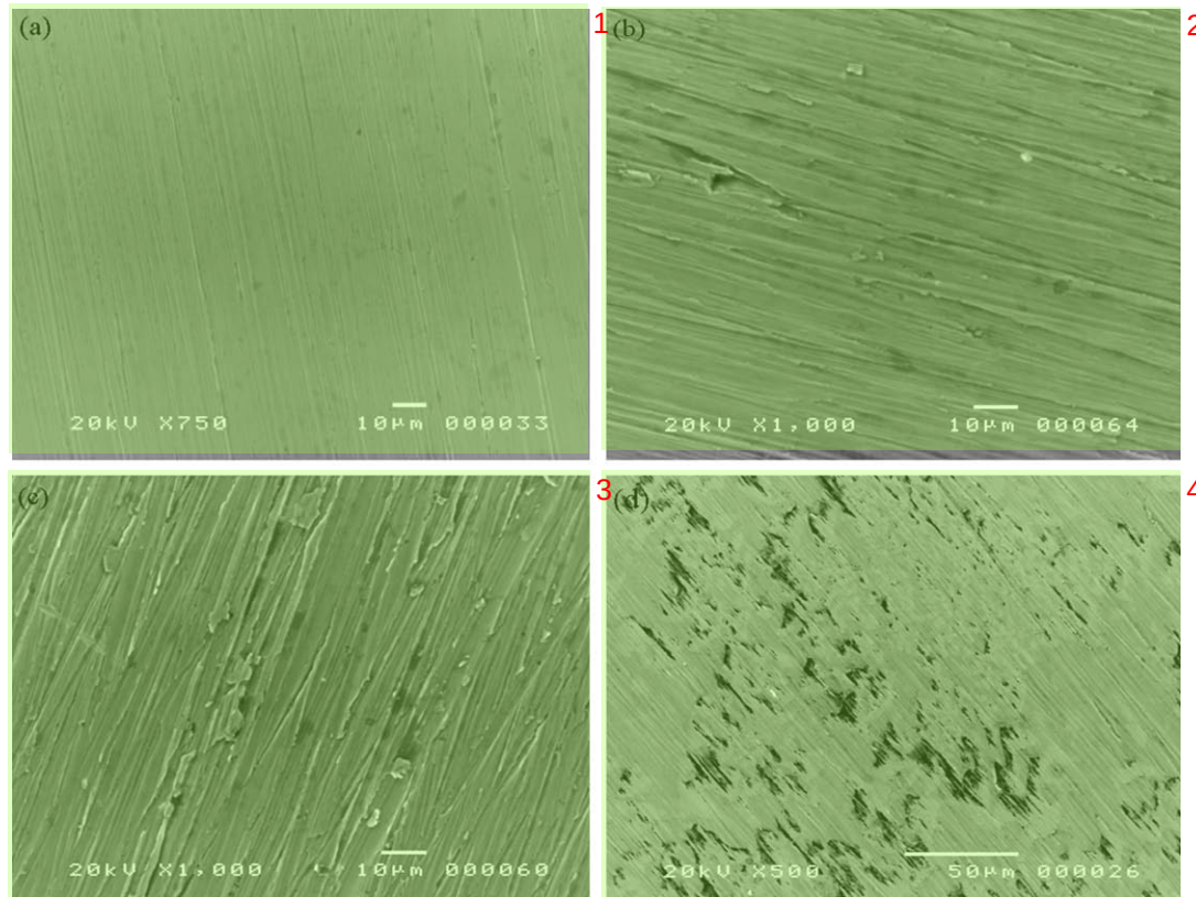
Fig. 8. SEM images of the \text{Co}_{1.5}\text{CrFeNi}_{1.5}\text{Ti}_{0.5}\text{Mo}_x high-entropy alloys: (a) x = 0 , (b) x = 0.1 , (c) x = 0.5 , and (d) x = 0.8 mol after potentiodynamic polarisation in deaerated 1 M NaOH.
