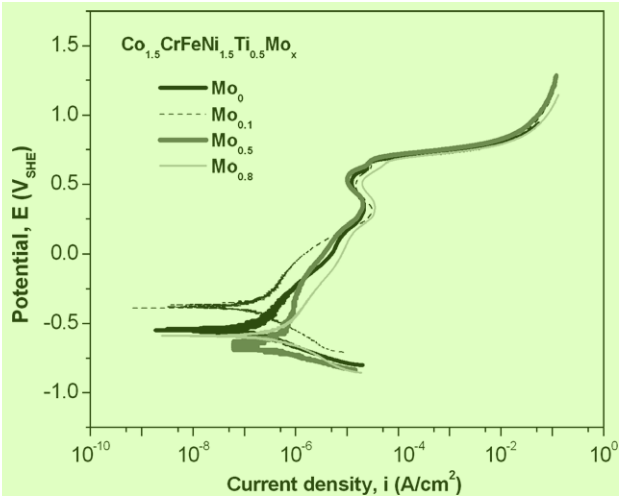
Fig. 4. Potentiodynamic polarisation curves of the Co 1.5 CrFeNi 1.5 Ti 0.5 Mo x alloys with various Mo contents ( x = 0 , x = 0.1 , x = 0.5 , and x = 0.8 mol) in deaerated 1 M NaOH.
